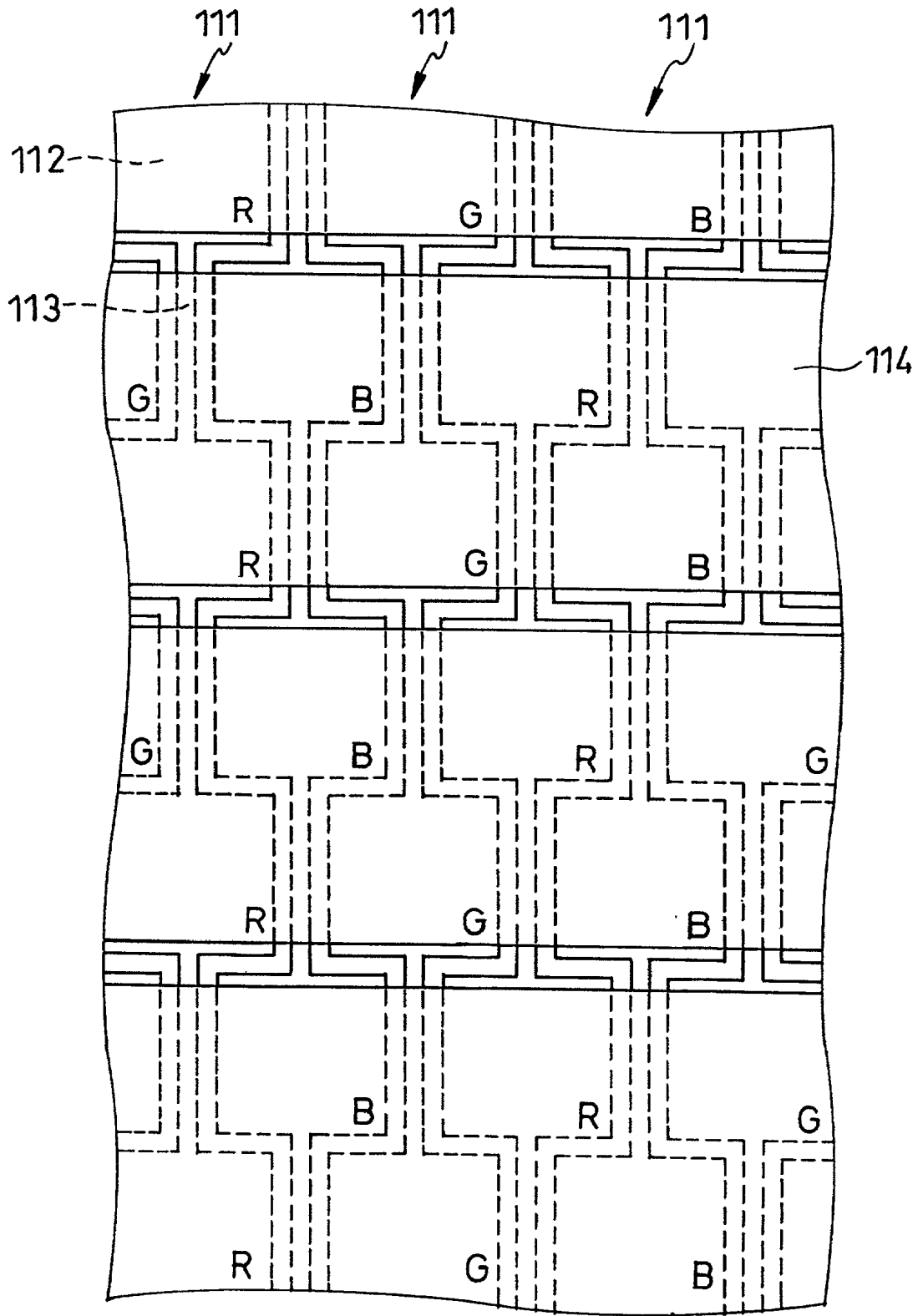
FIG. 3 (PRIOR ART)
